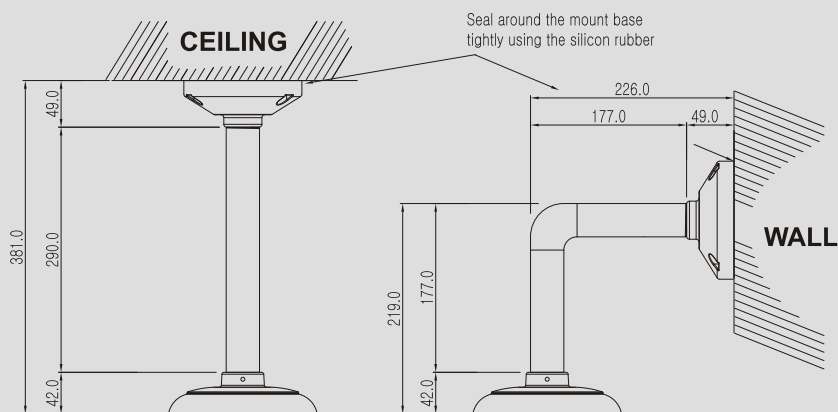
[ Dimension Drawing ]
