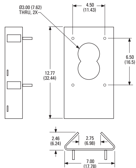
NOTE: VALUES IN PARENTHESES ARE CENTIMETERS; ALL OTHERS ARE INCHES.
