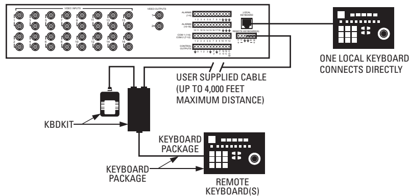
SAMPLE CM6700 KEYBOARD WIRING DIAGRAM
