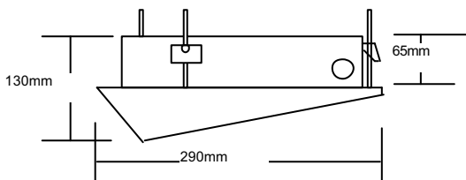
RMW2 Recess Mount Wedge Housing
